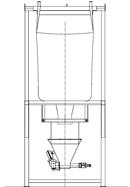
Adjustable big bag support stand with multiscrew feeder.
